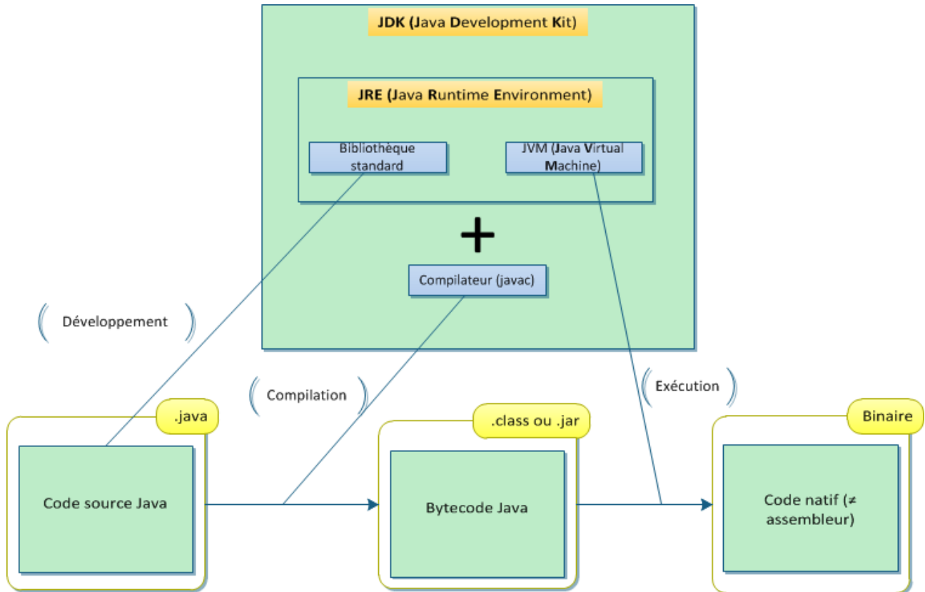
FIGURE 30.2. – Architecture Java
