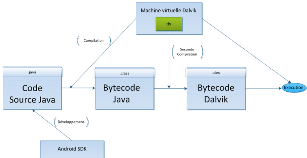
FIGURE 30.3. – Dalvik
